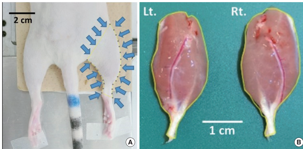
Supplementary Fig. 1. An analytical way of dimension measurements at both bilateral hind-limb and gastrocnemius. (A) A example of region to measure right hind-limb dimension (yellow line and blue arrows). (B) A example of region to measure both sides of gastrocnemius muscle (yellow lines). Lt., left; Rt., right.
